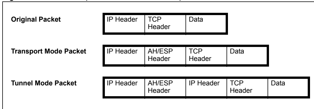
Figure 132 VPN: Transport and Tunnel Mode Encapsulation
