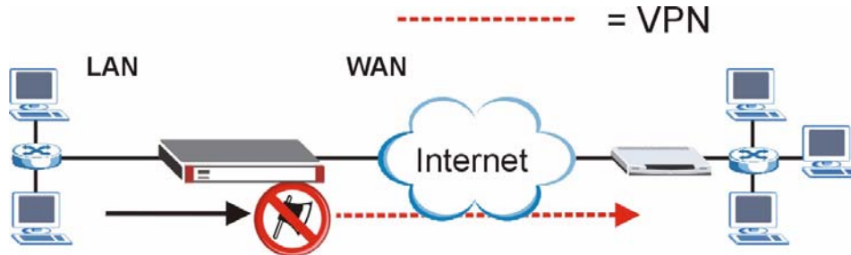
Figure 44 Tutorial: IDP for To VPN Traffic
