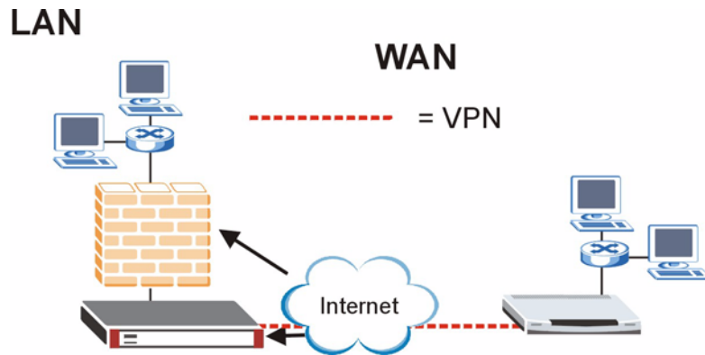
Figure 77 From VPN to LAN Example
