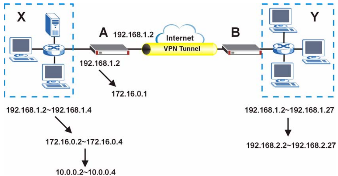
Figure 131 Virtual Mapping of Local and Remote Network IP Addresses
