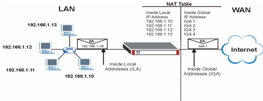
Figure 166 How NAT Works
