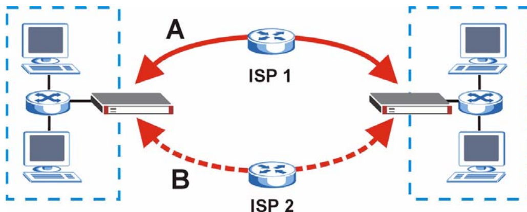
Figure 128 IPsec High Availability
