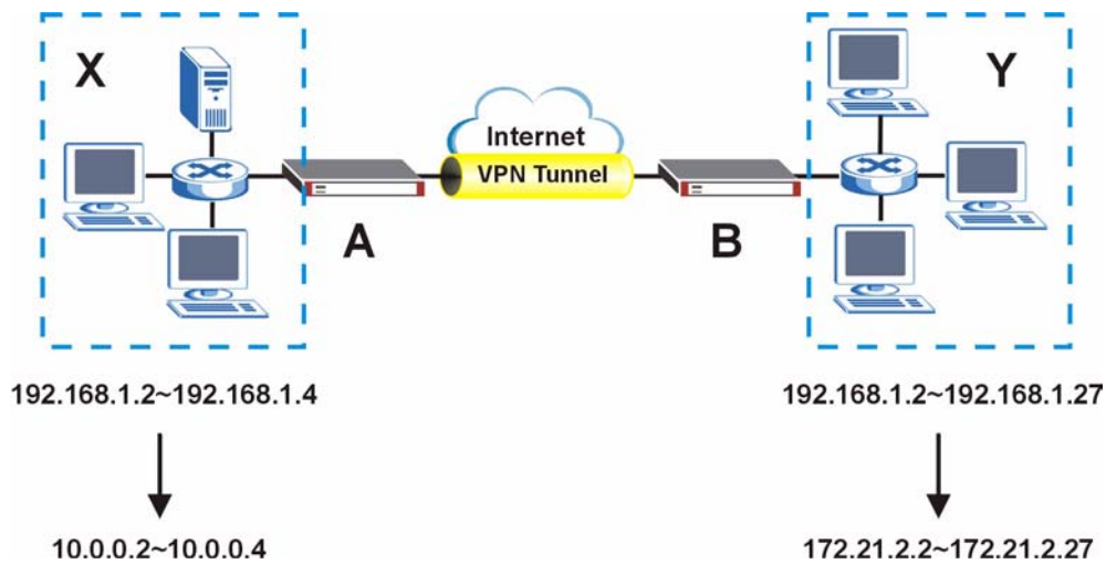
Figure 130 Virtual Mapping of Local and Remote Network IP Addresses
