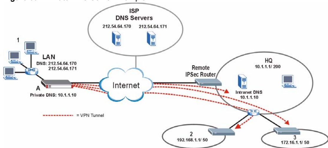
Figure 59 Private DNS Server Example
