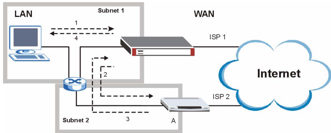
Figure 83 Using IP Alias to Solve the Triangle Route Problem
