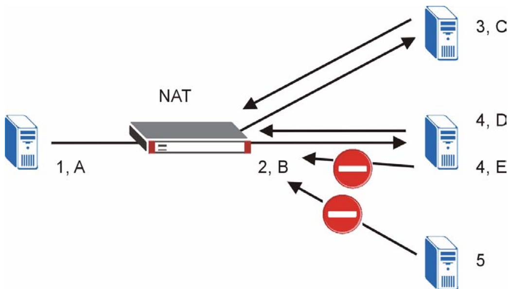
Figure 168 Port Restricted Cone NAT Example
