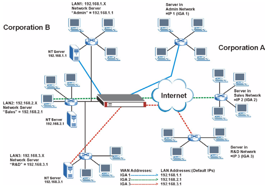
Figure 167 NAT Application With IP Alias
