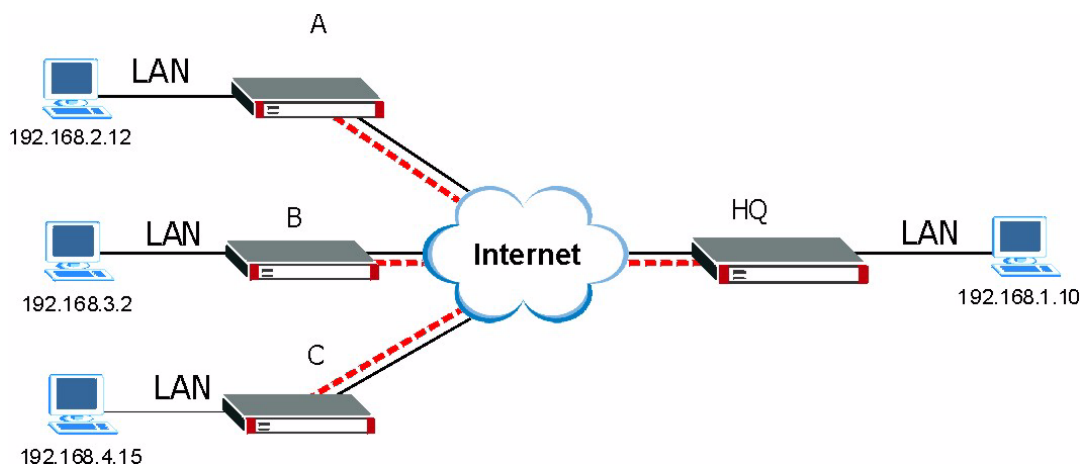
Figure 144 Telecommuters Sharing One VPN Rule Example
