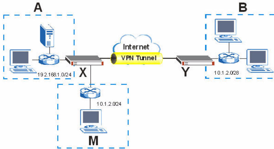
Figure 142 Overlap in IP Alias and VPN Remote Networks
