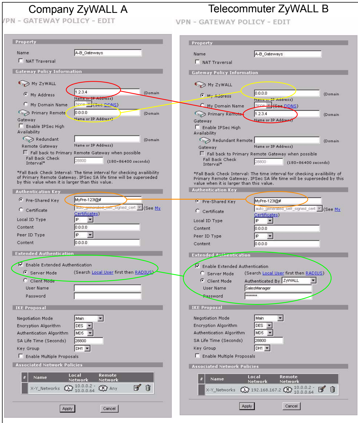
Figure 35 VPN Gateway Policy Edit Screens
