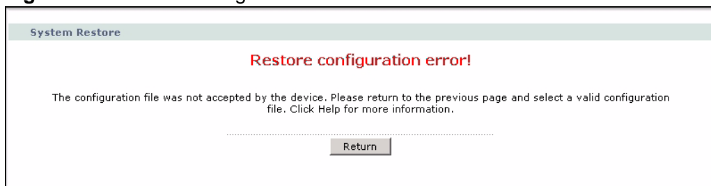
Figure 127 Error Message
