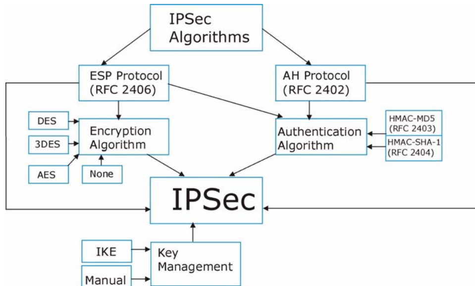
Figure 77 IPSec Architecture
