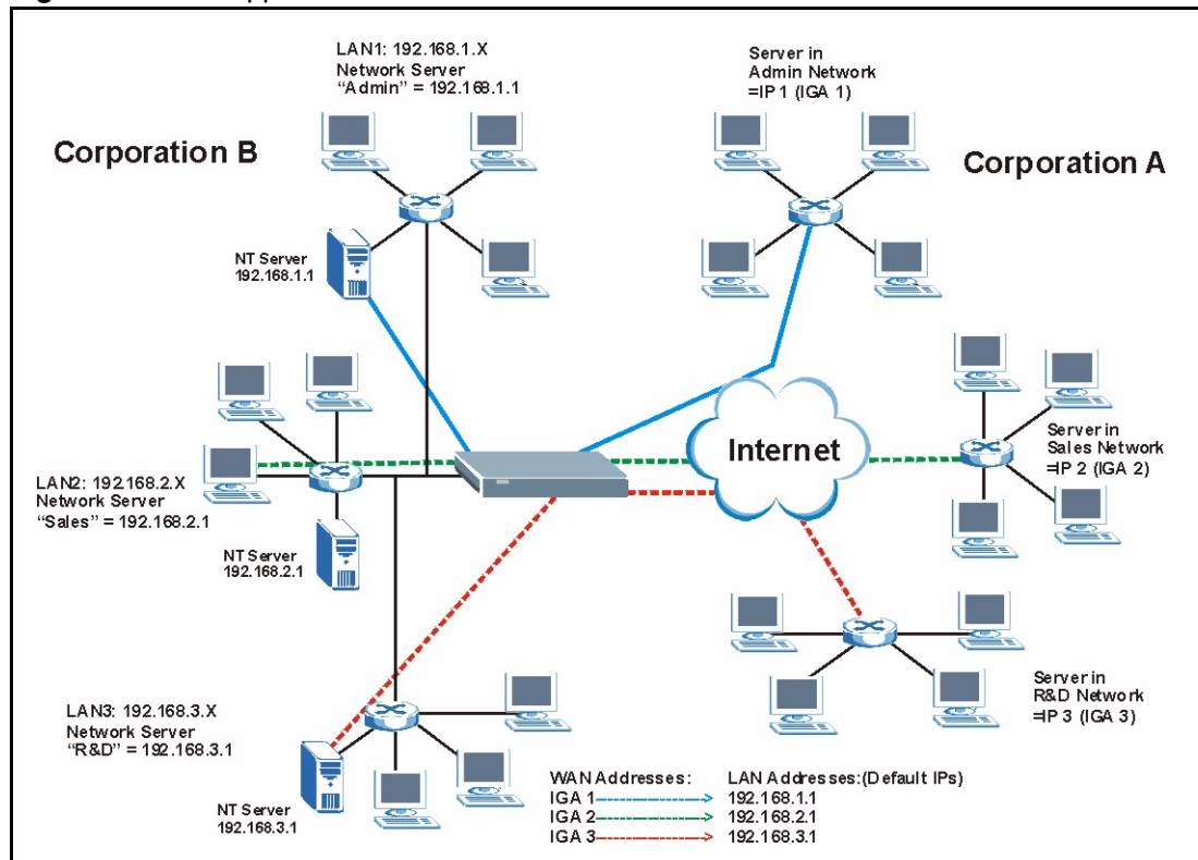
Figure 28 NAT Application With IP Alias
