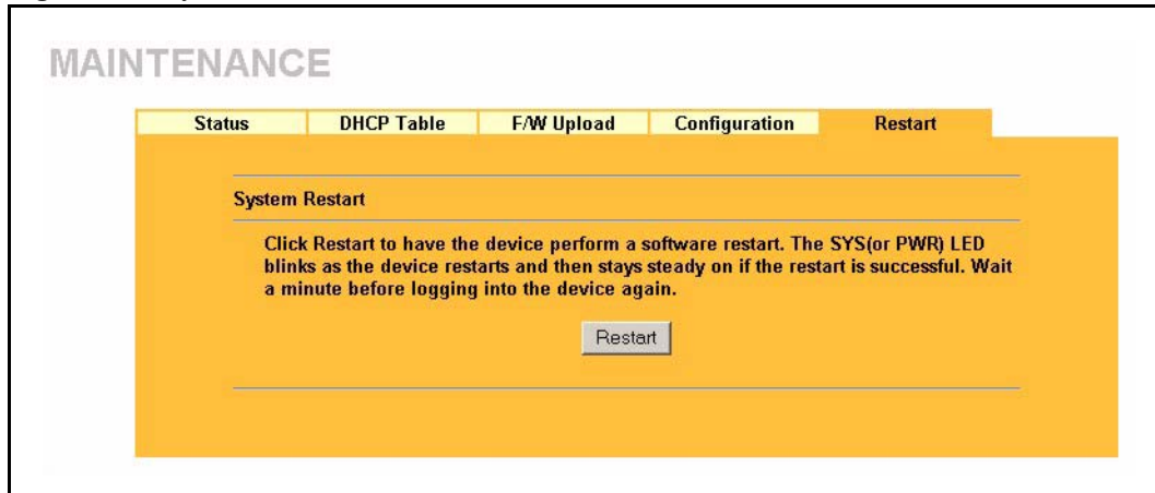
Figure 86 System Restart
