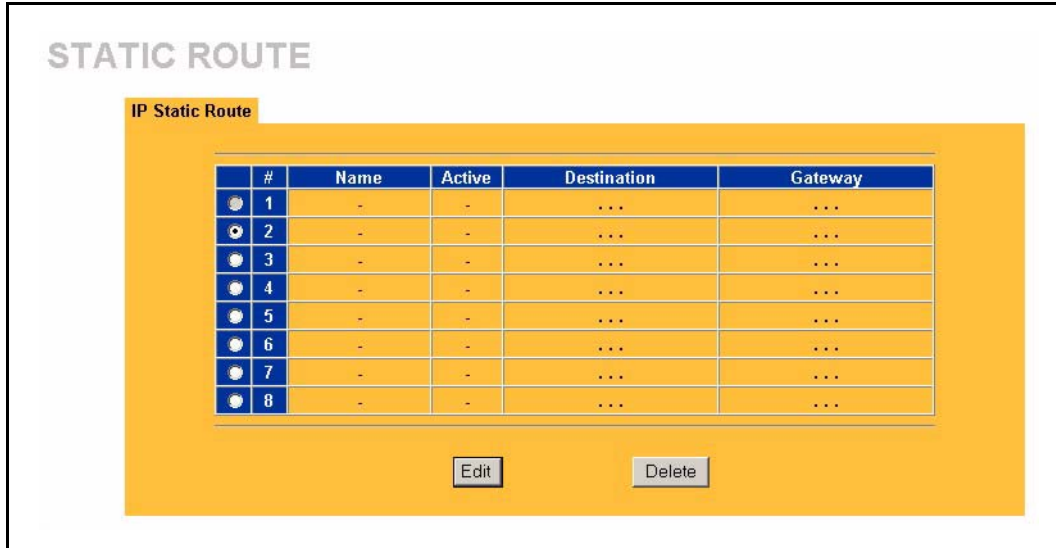
Figure 36 Static Route
