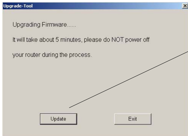
Figure 78 Upgrade Tool
