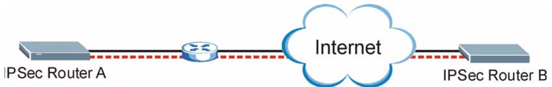
Figure 94 NAT Router Between IPsec Routers
