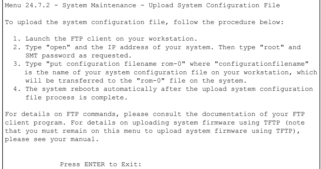
Figure 239 Telnet Into Menu 24.7.2 System Maintenance
