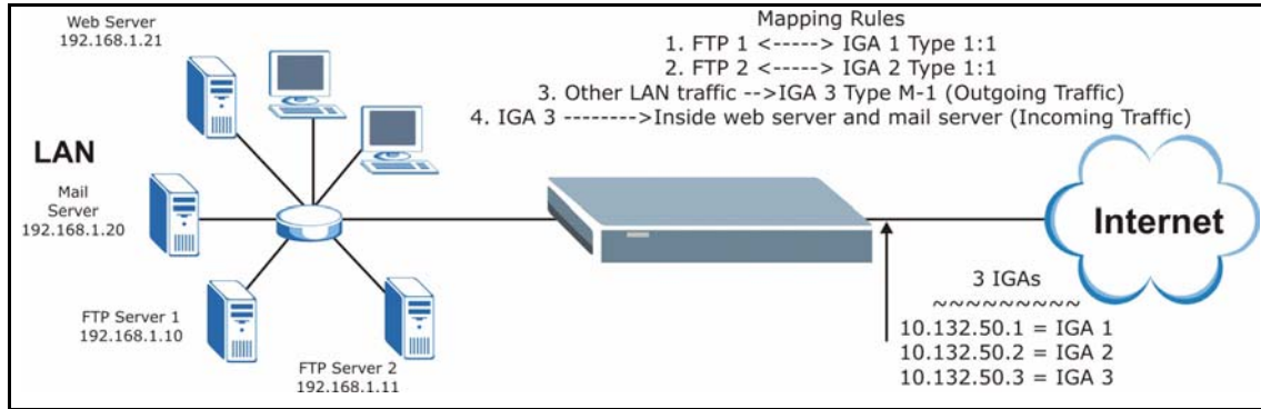
Figure 191 NAT Example 3
