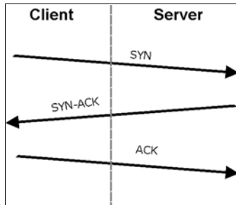
Figure 67 Three-Way Handshake
