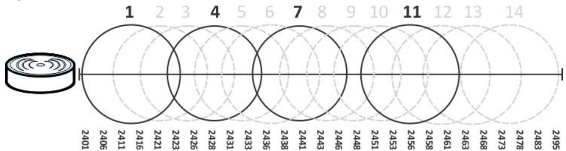
Figure 54 An Example Four-Channel Deployment
