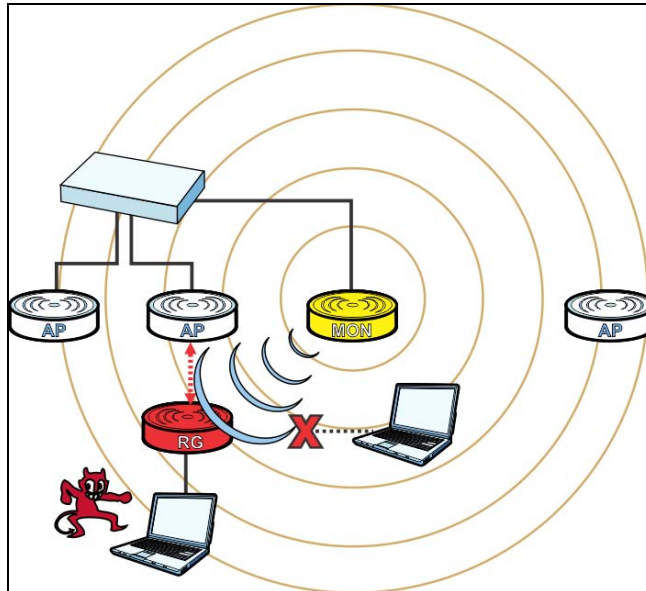
Figure 22 Containing a Rogue AP
