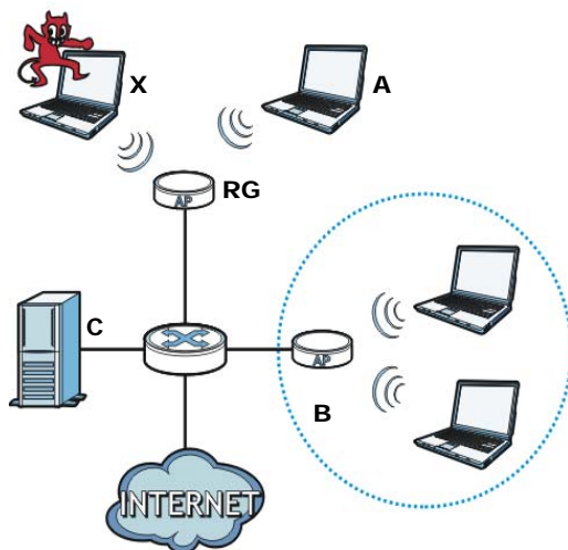
Figure 76 Rogue AP Example
