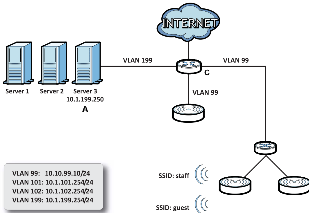
Figure 18 Tutorial Network Topology
