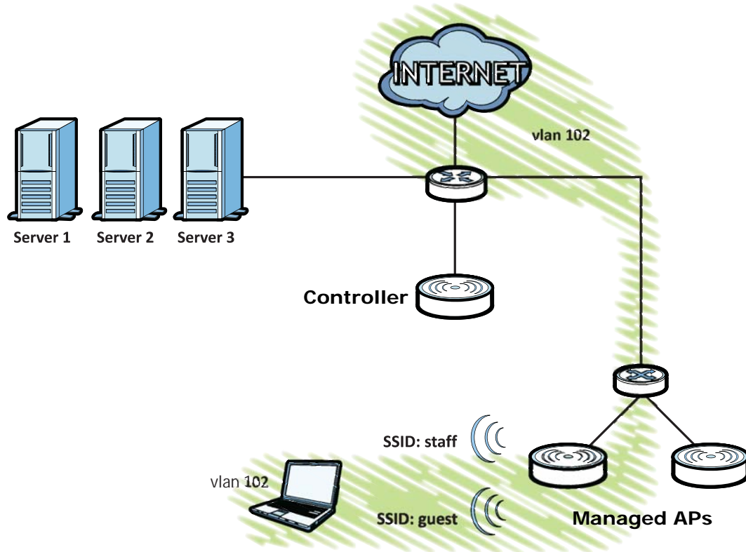
Figure 19 Tutorial Guest VLAN Example
