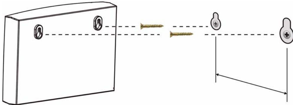
Figure 125 Wall-mounting Example
