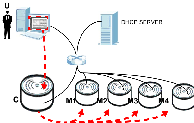
Figure 38 CAPWAP Network Example
