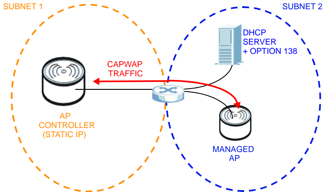
Figure 39 CAPWAP and DHCP Option 138
