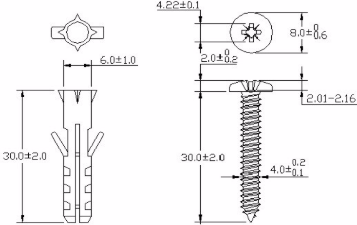
Figure 126 Masonry Plug and M4 Tap Screw
