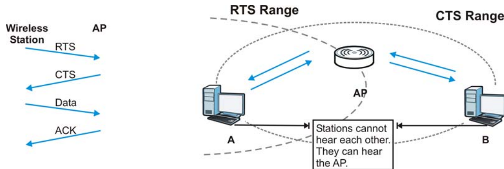
Figure 130 RTS/CTS
