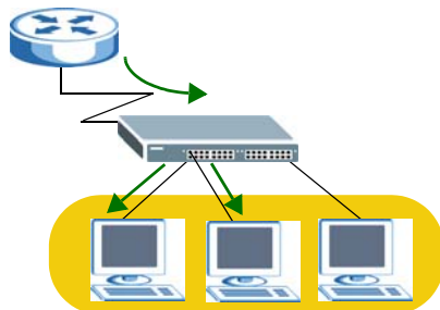
Figure 63 Static Multicast Forwarding to Multiple Ports
