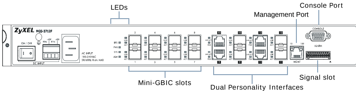
Figure 9 Front Panel: MGS-3712F
