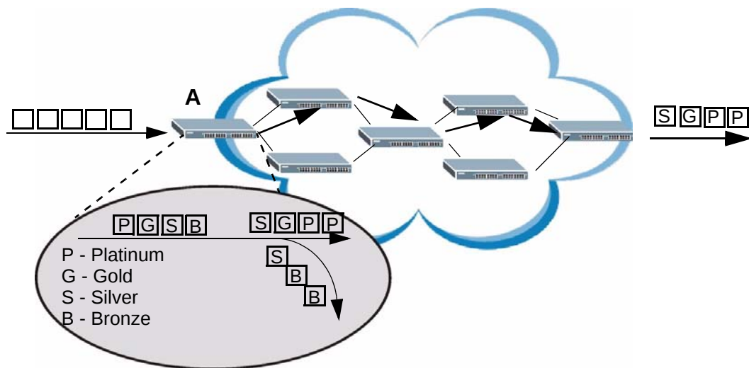
Figure 150 DiffServ Network
