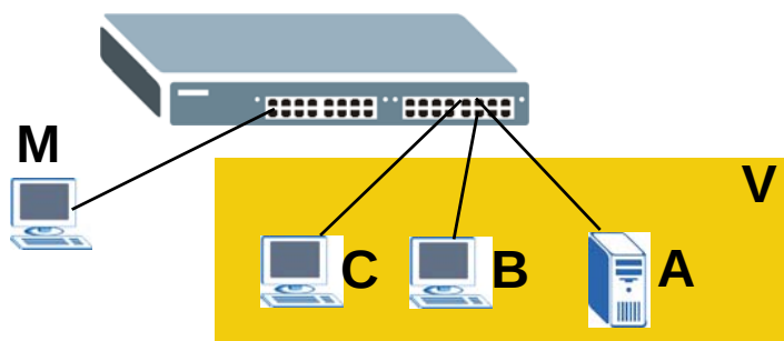
Figure 19 Tutorial: DHCP Snooping Tutorial Overview
