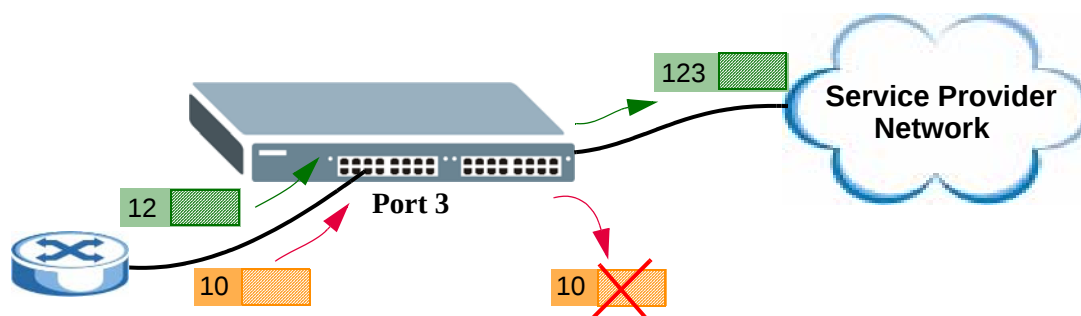
Figure 141 VLAN mapping example
