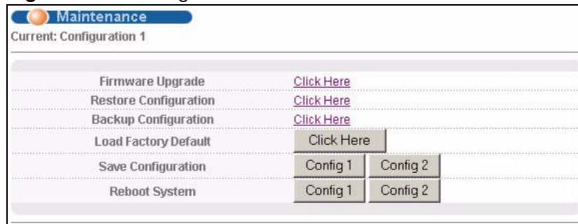
Figure 163 Management > Maintenance
