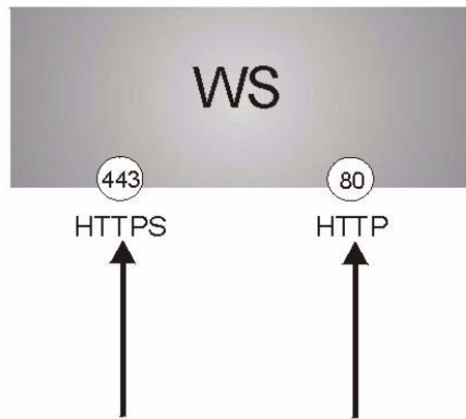
Figure 176 HTTPS Implementation
