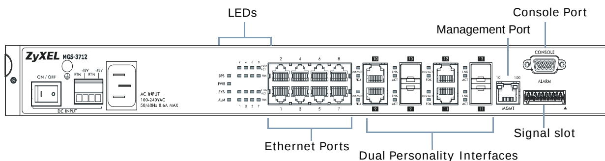
Figure 8 Front Panel: MGS-3712
