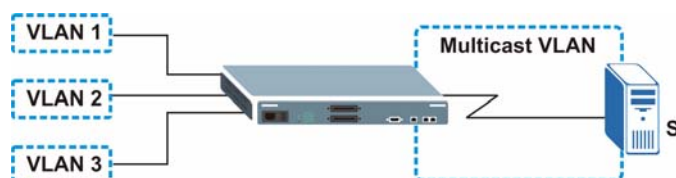
Figure 109 MVR Network Example
