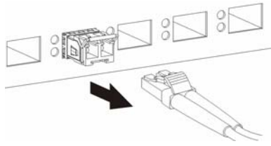
Figure 13 Opening the Transceiver's Latch Example
