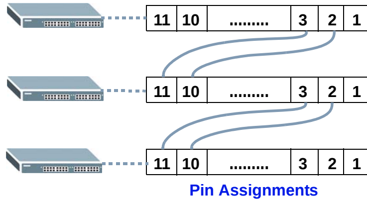
Figure 16 Daisy-chaining an External Alarm Sensor to Other Switches of the Same Model
