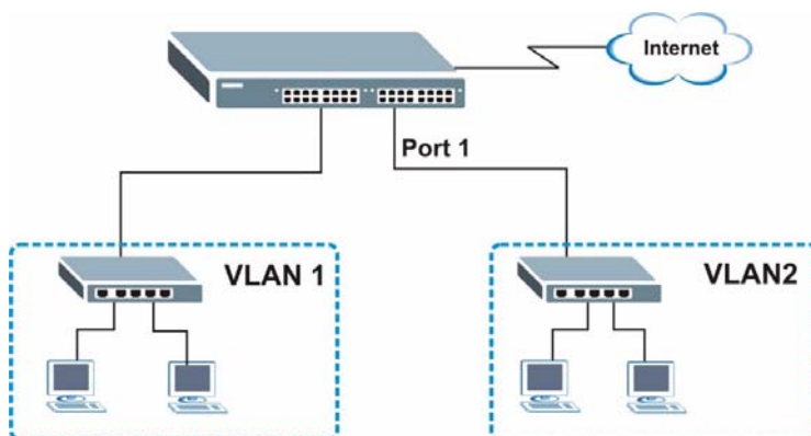
Figure 37 Initial Setup Network Example: VLAN
