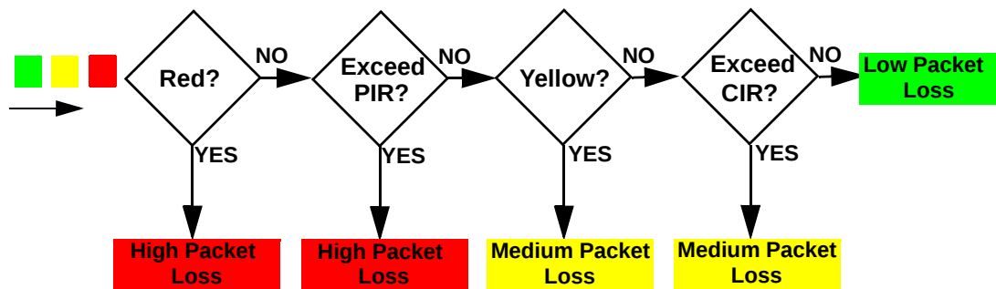
Figure 152 TRTCM-Color-aware Mode
