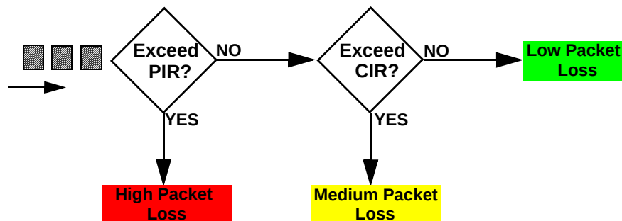
Figure 151 TRTCM-Color-blind Mode
