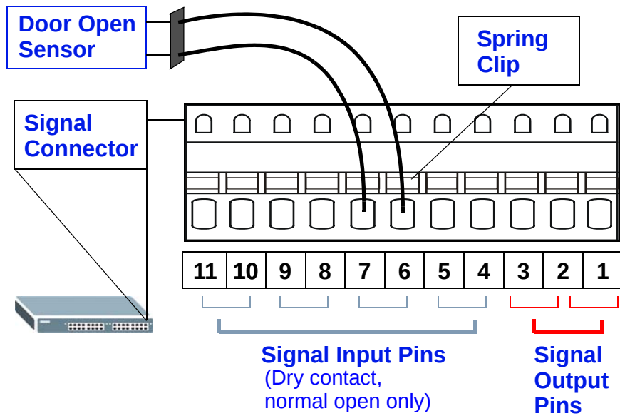
Figure 15 Connecting a Sensor to the Signal Slot
