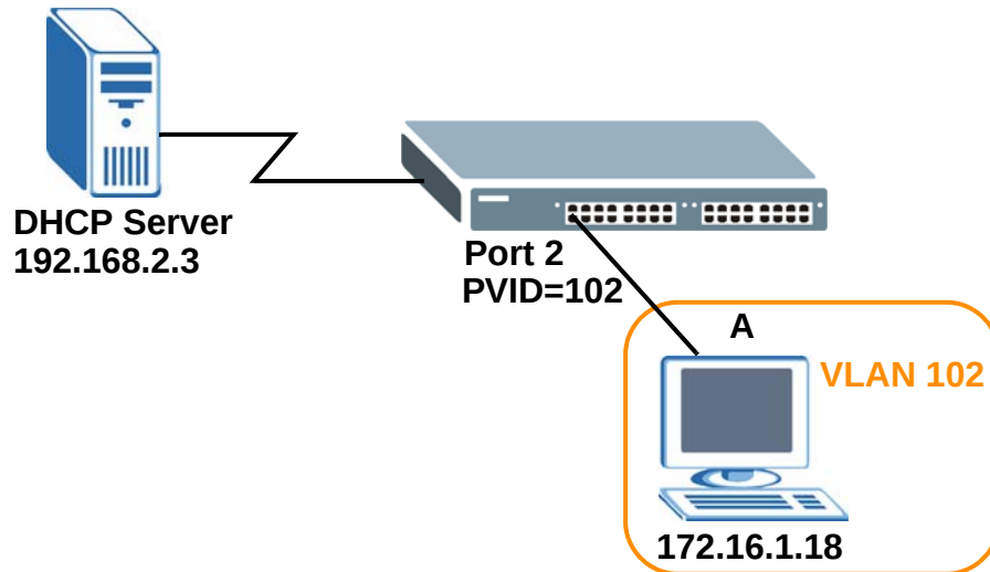
Figure 26 Tutorial: DHCP Relay Scenario
