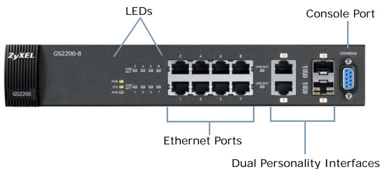
Figure 9 Front Panel (GS2200-8)
