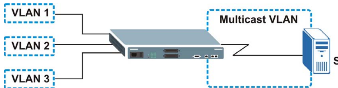
Figure 103 MVR Network Example
