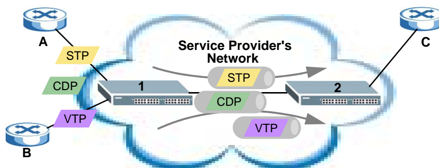
Figure 139 Layer 2 Protocol Tunneling Network Scenario
