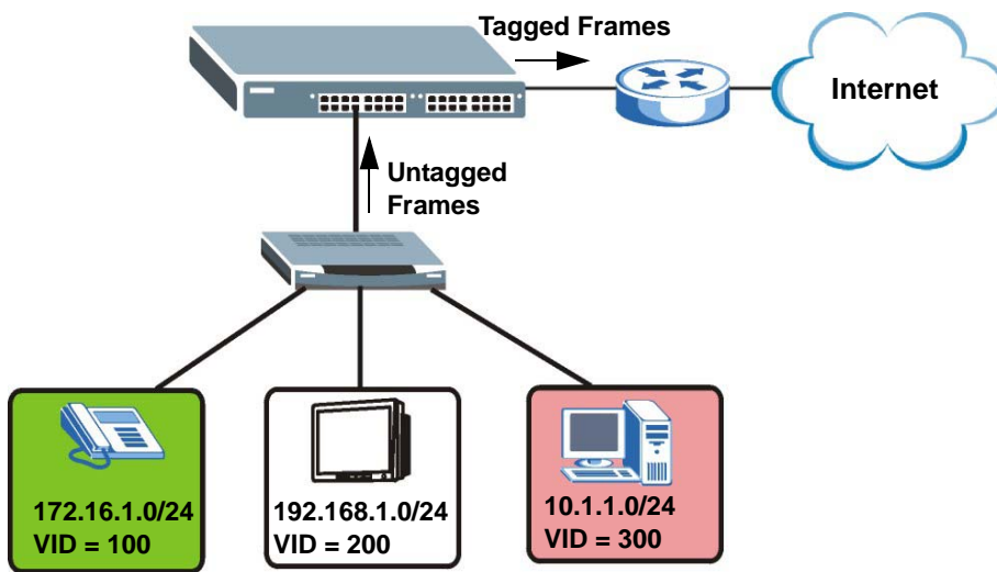
Figure 55 Subnet Based VLAN Application Example
