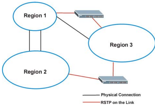
Figure 81 MSTP and Legacy RSTP Network Example
