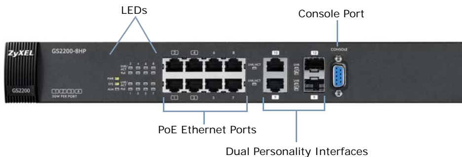
Figure 10 Front Panel (GS2200-8HP)
