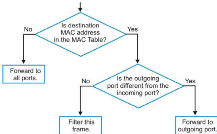
Figure 197 MAC Table Flowchart
