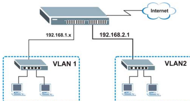
Figure 24 Initial Setup Example: Management IP Address
