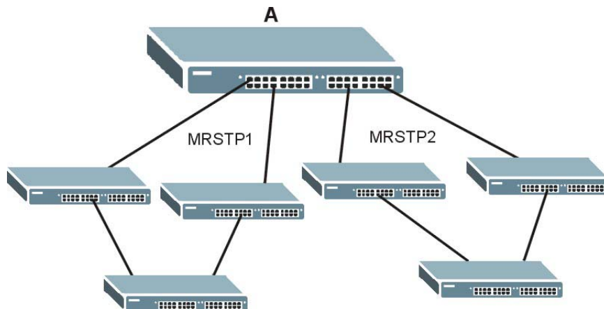
Figure 68 MRSTP Network Example
