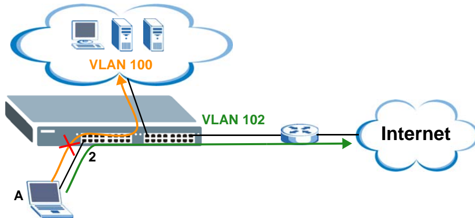
Figure 93 Guest VLAN Example
