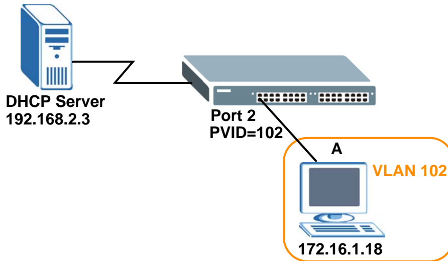
Figure 32 Tutorial: DHCP Relay Scenario
