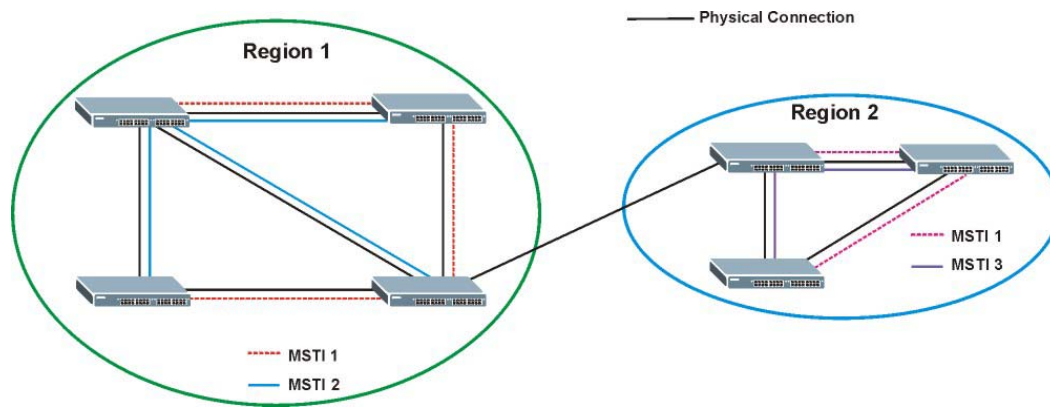
Figure 80 MSTIs in Different Regions
