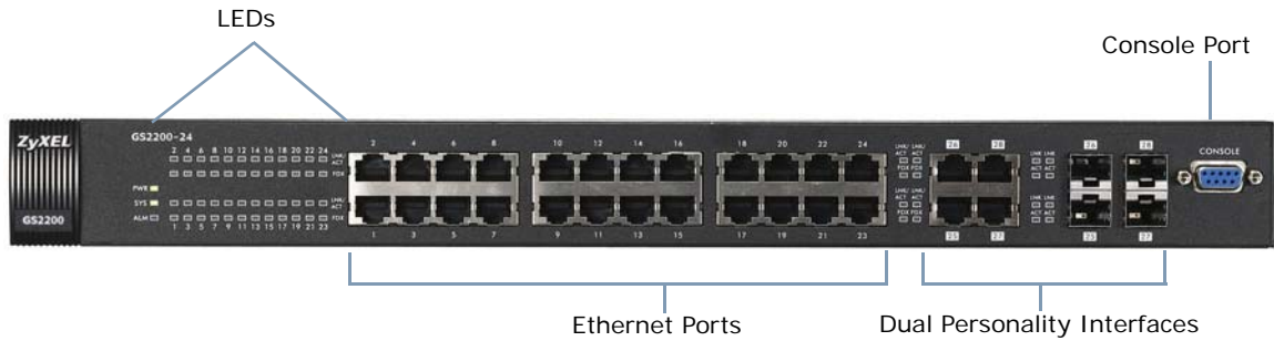
Figure 11 Front Panel (GS2200-24)
