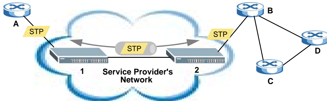
Figure 140 L2PT Network Example
