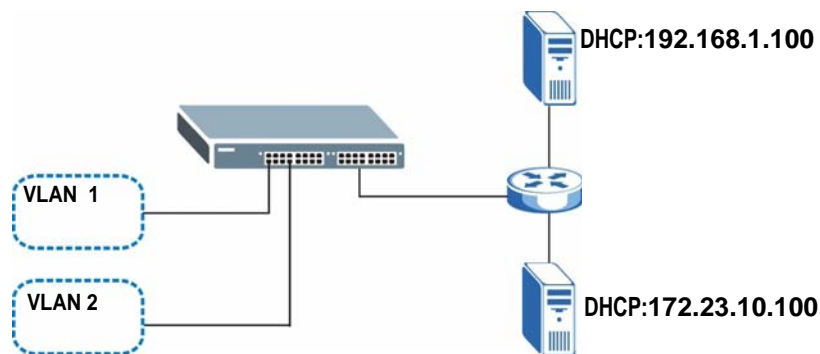
Figure 162 DHCP Relay for Two VLANs
