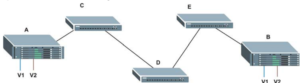
Figure 49 Port VLAN Trunking
