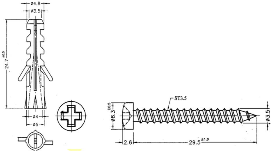
Figure 8 Masonry Plug and 3.5 mm Self-Tapping Screw
