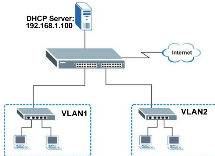
Figure 159 Global DHCP Relay Network Example
