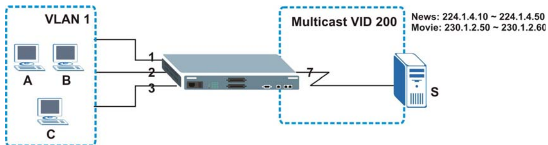
Figure 111 MVR Configuration Example
