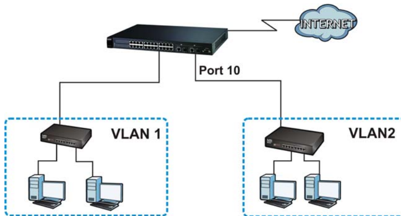
Figure 21 Initial Setup Network Example: VLAN
