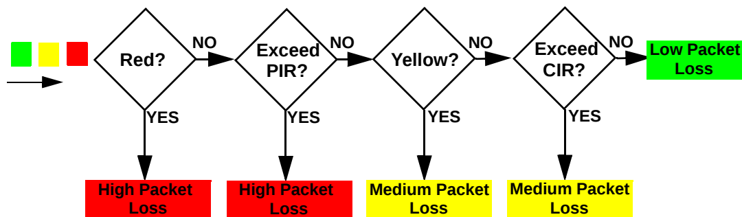
Figure 160 TRTCM-Color-aware Mode
