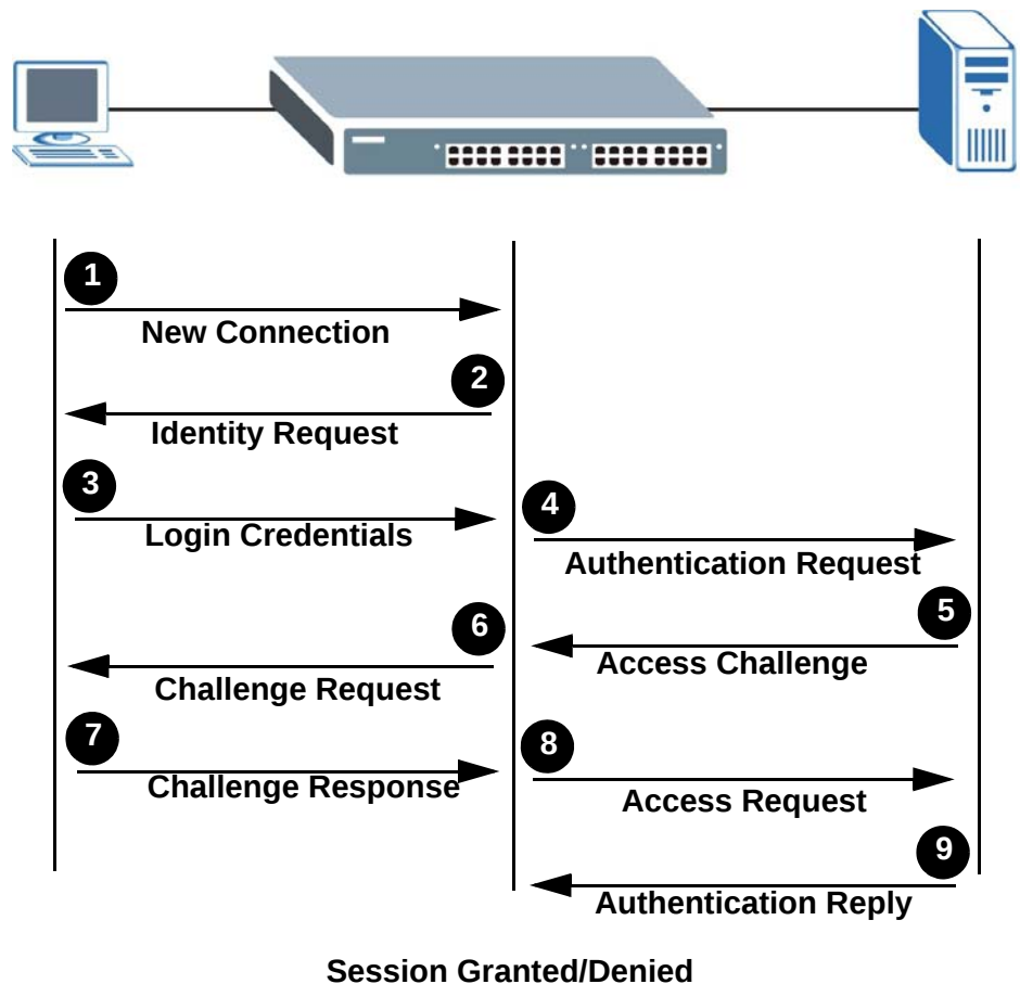
Figure 79 IEEE 802.1x Authentication Process
