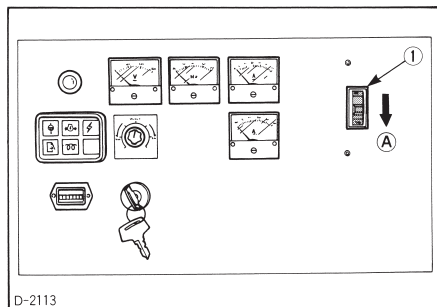
(1) Interruptor principal (llave)
