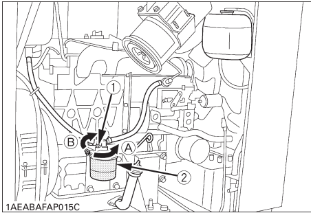
1AEABAFAP015C (1) Air bleeding cock (A) "OPEN" (2) Fuel filter cartridge (B) "CLOSE"
