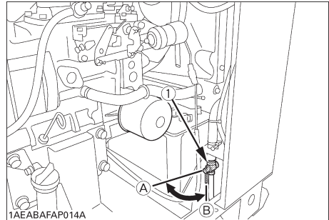
(1) Water drain cock (A) "OPEN" (B) "CLOSE"
