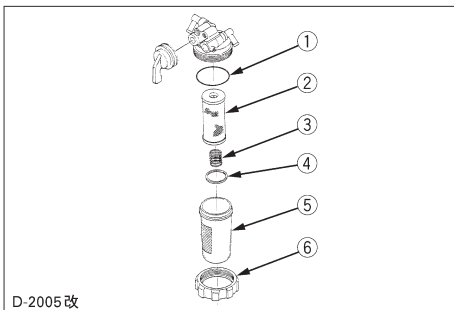
(1) Joint torique
