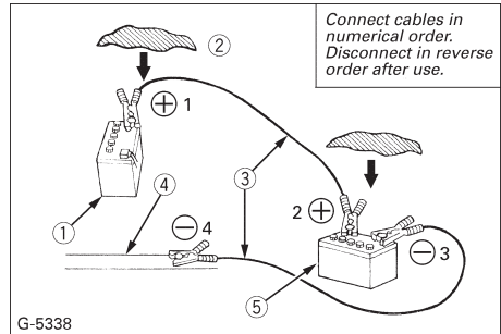
(1) Dead battery
