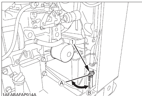
1AFA8AFAP014A (1) 放水螺塞 (A) “开” (B) “闭”
