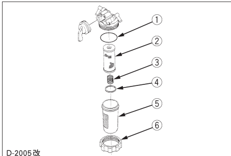
(1) O ring (2) Filter element (3) Spring (4) Marker (5) Filter bowl (6) Screw ring
