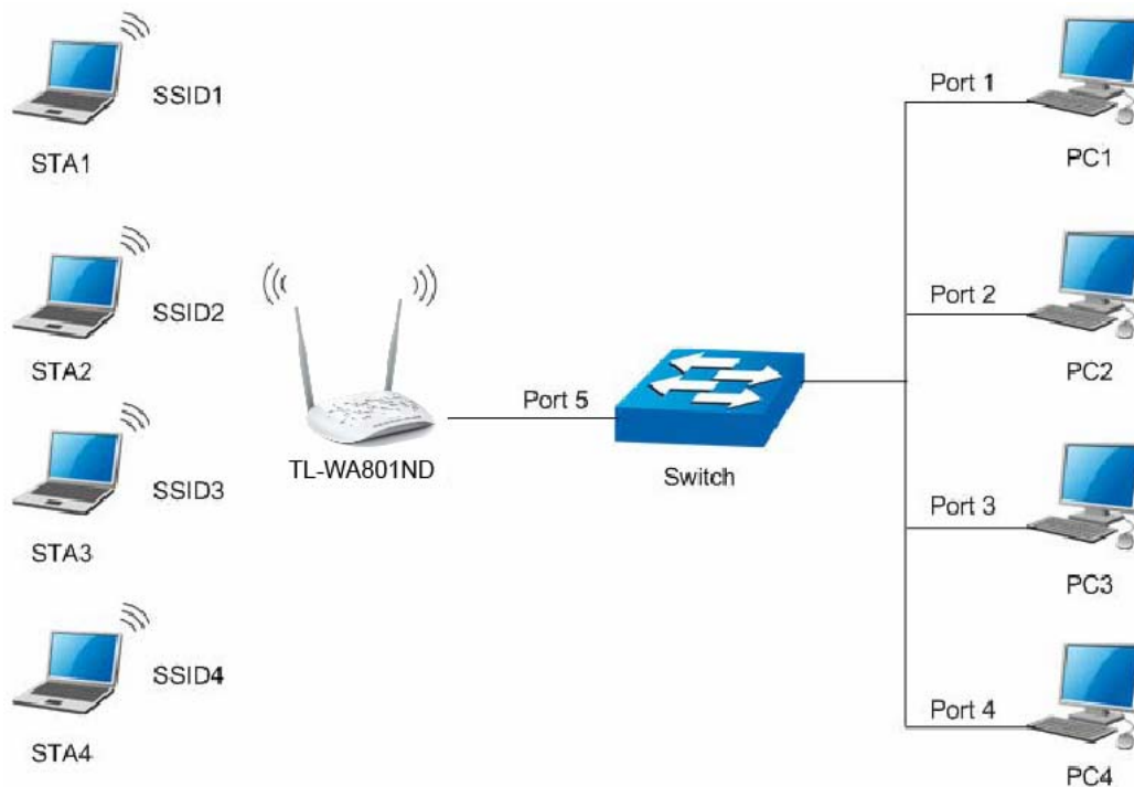
Multi-SSID+VLAN
