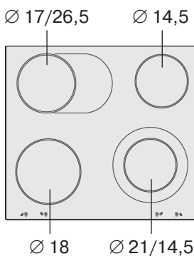
EA6..GN..
