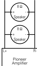
4 Ω Bridged Mode
