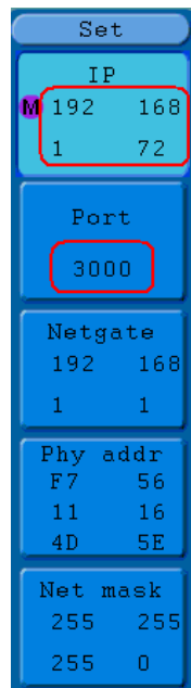
Figure 6-4 Set the network parameters of the oscilloscope
