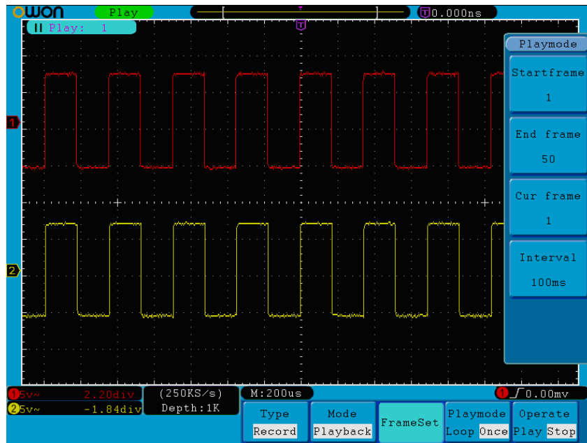
Figure 5-38 Wave Playback
