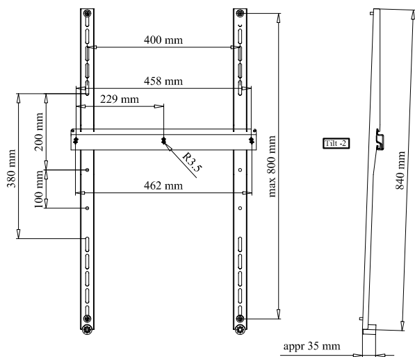
NEC WS32-52P - 100012665 Portrait Dimensions:
