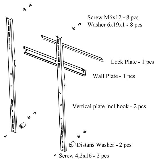
NEC WS32-52P - 100012665 Portrait Box Contains:
