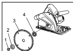
1. Perno hexagonal 2. Brida exterior 3. Disco de sierra 4. Brida interior
