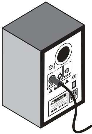
balanced connection
