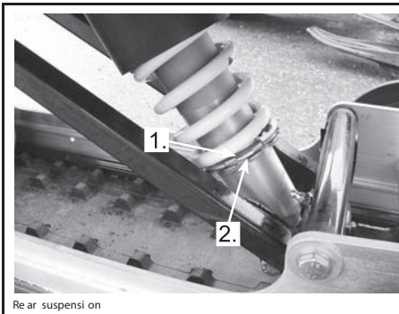
Rear suspension
