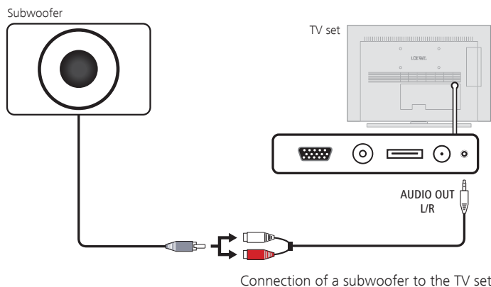
Connection of a subwoofer to the TV set
