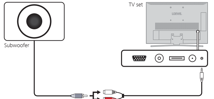
Connection of a subwoofer to the TV set
