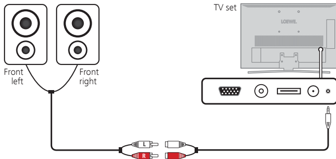
Connection of active speakers to the TV set
