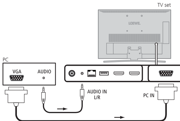
Connection example of a PC
