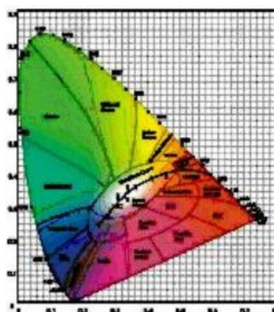
CIE1931
