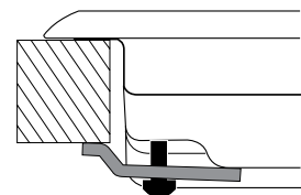
Hooking position for top H=30mm
