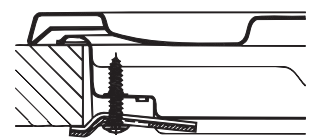
Hooking position for top H=30mm
