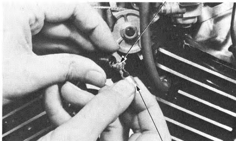
(2) CHOKE VALVE
