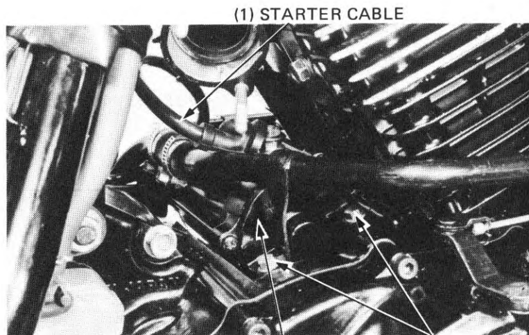
(2) STARTER MOTOR (3) BOLTS
