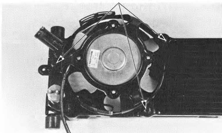
(1) MOUNTING BOLTS
