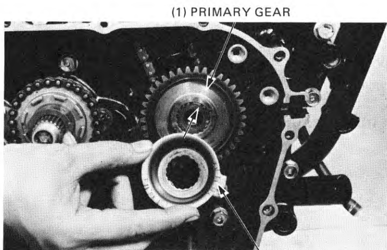
(1) PRIMARY GEAR (2) PULSE GENERATOR PLATE
