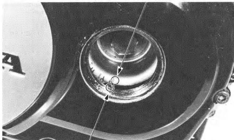
(2) INDEX MARK
