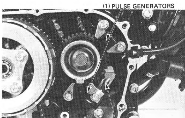
(2) WIRE CLAMP
