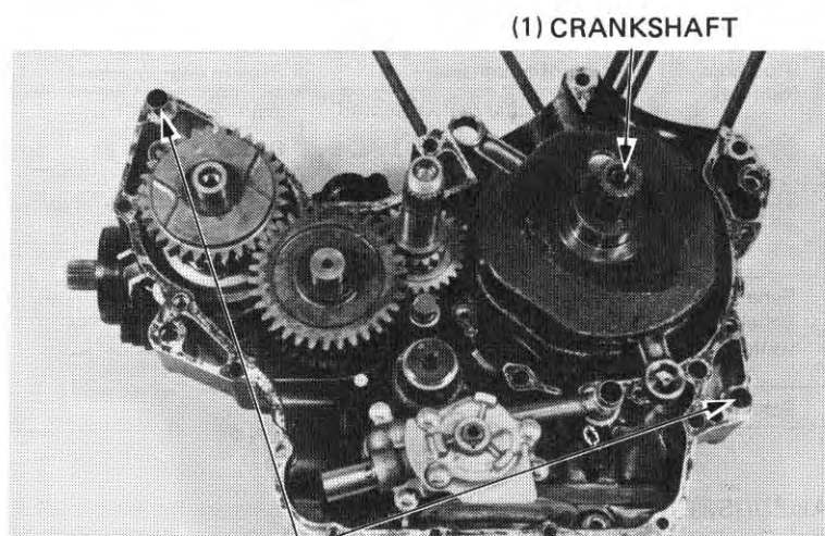
(2) DOWEL PINS
