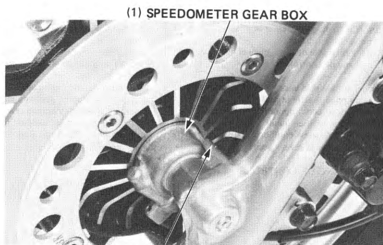
(2) BOSS
