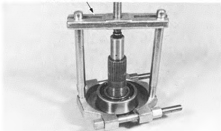
(1) BEARING PULLER
