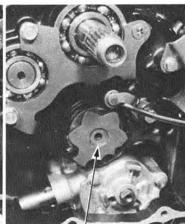
(3) STOPPER PLATE
