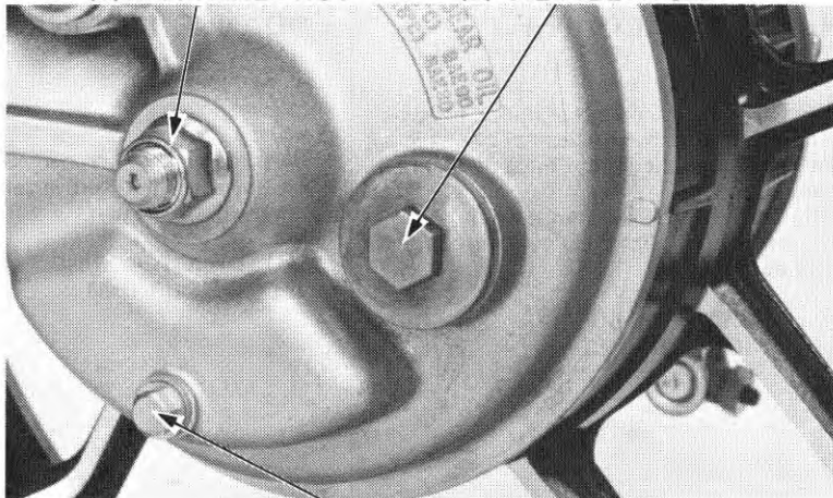
(3) DRAIN BOLT
