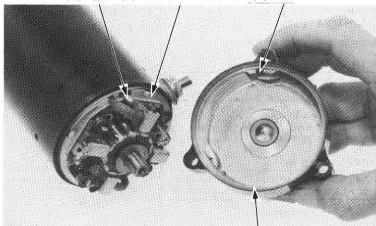
(4) REAR BRACKET
