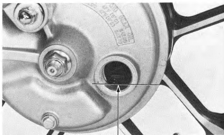
(3) OIL LEVEL
