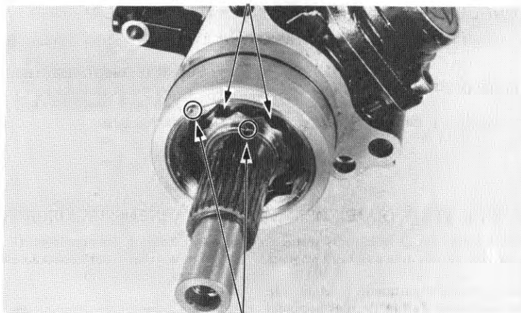
(2) UNSTAKE
