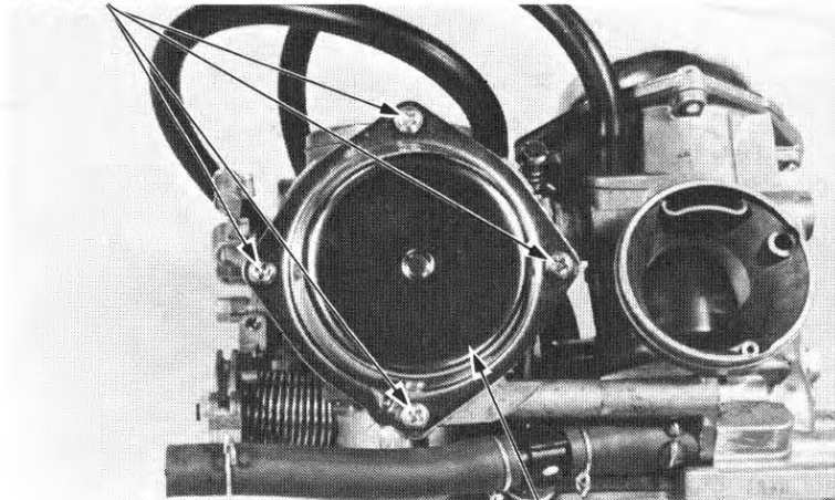
(2) COVER
