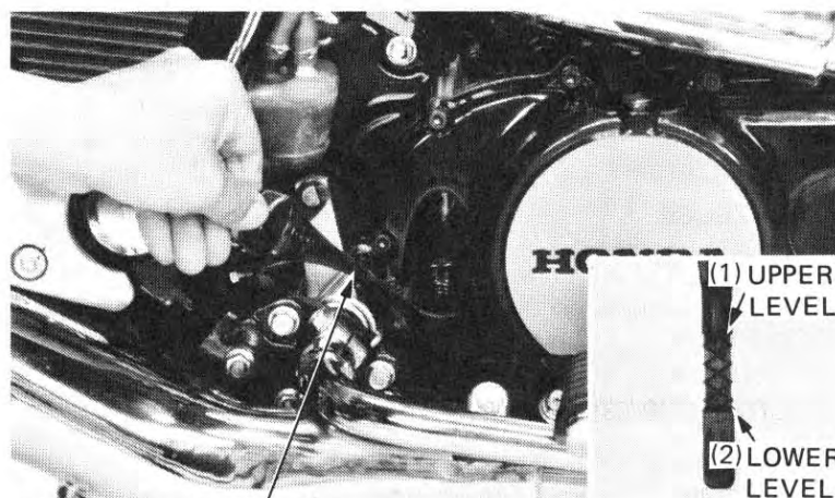
(3) OIL FILTER/DIPSTICK
