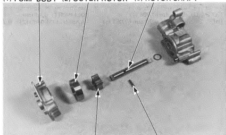
(4) INNER ROTOR (5) DRIVE PIN
