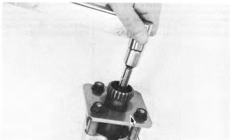
(1) PINION HOLDER 07924-ME40000
