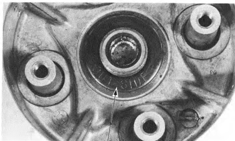
(1) LOCK WASHER
