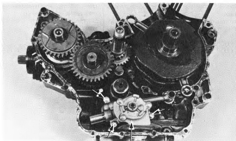
(1) OIL PUMP
