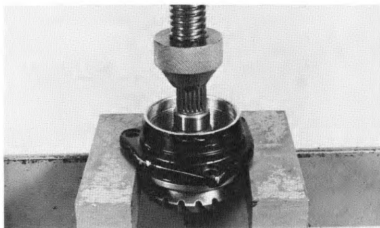
(1) DRIVER A 07749-0010000
