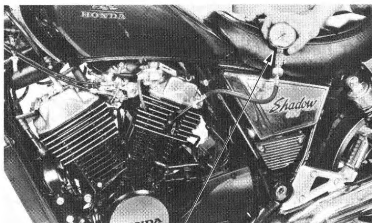
(1) COMPRESSION GAUGE
