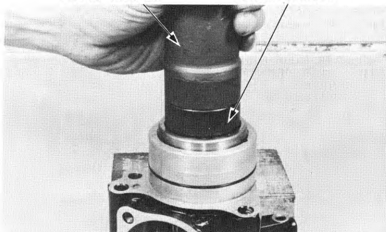
(1) DRIVER C 07746-0020100
