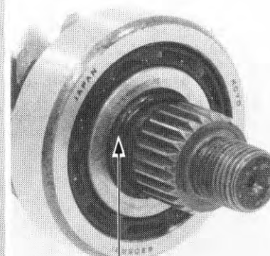
(2) O-RING
