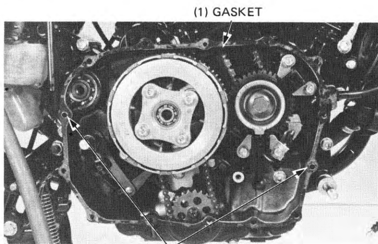
(1) GASKET (2) DOWEL PINS
