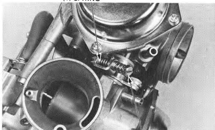
(2) ADJUSTING SCREW
