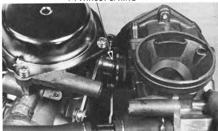
(1) THRUST SPRING
