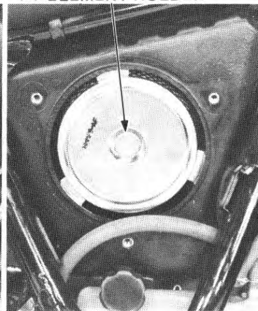
(3) ELEMENT HOLDER
