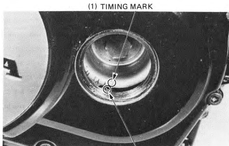
(2) INDEX MARK
