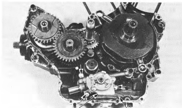
(1) OIL PUMP
