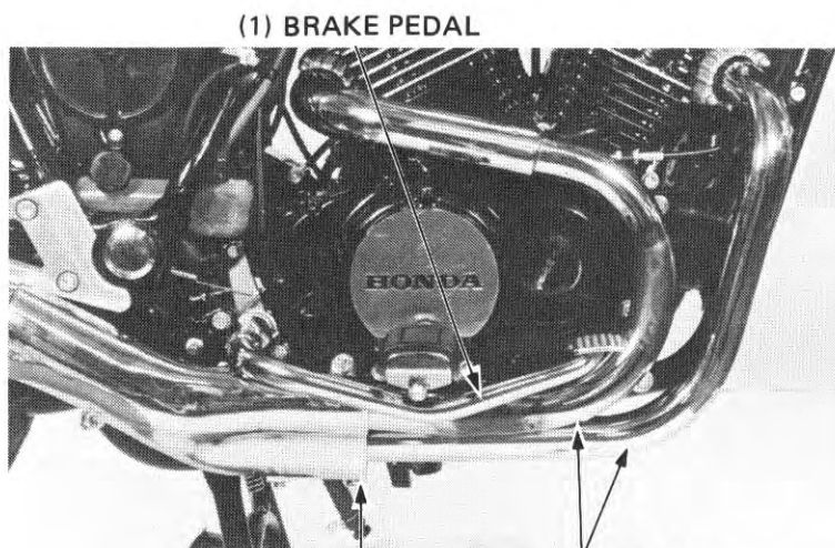
(2) CLAMP BOLT
