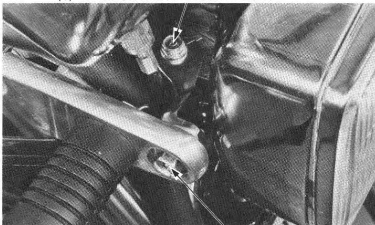
(2) MOUNTING BOLT
