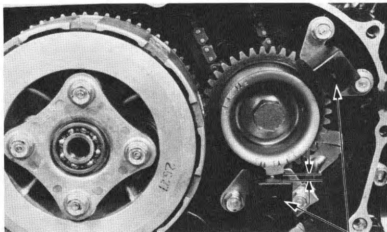
(1) PULSE GENERATOR
