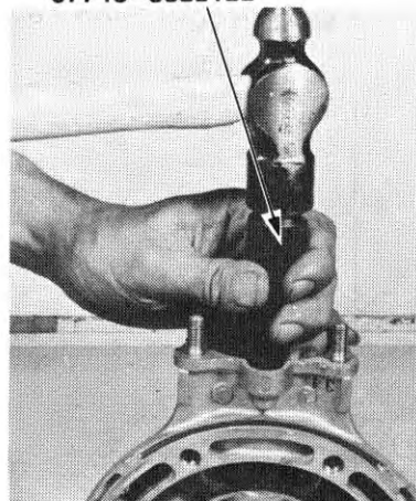
(1) DRIVER C 07746-0030100
