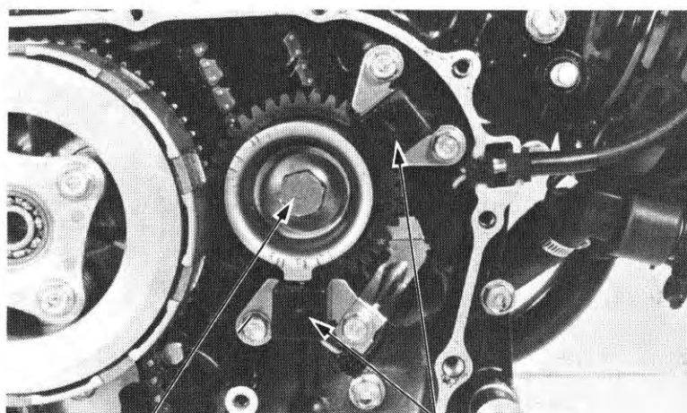
(1) GEAR BOLT (2) PULSE GENERATORS
