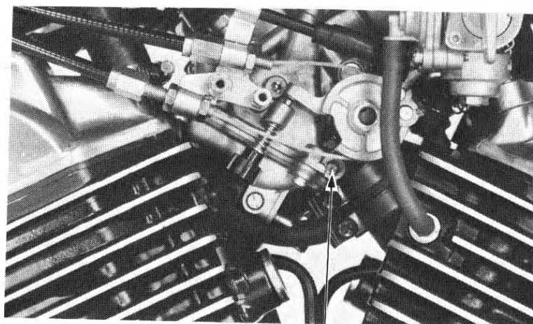
(1) PILOT SCREW
