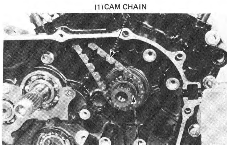
(2) TIMING SPROCKET
