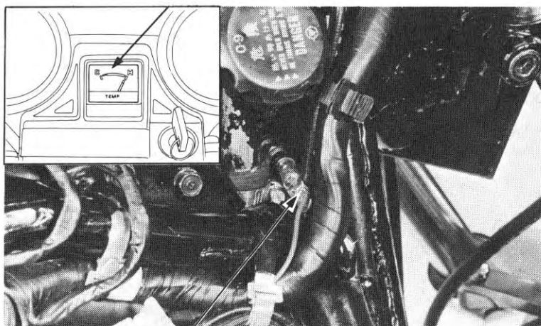
(2) TEMPERATURE SENSOR
