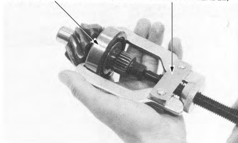
(1) PINION BEARING (2) BEARING PULLER (COMMERCIALLY AVAILABLE)
