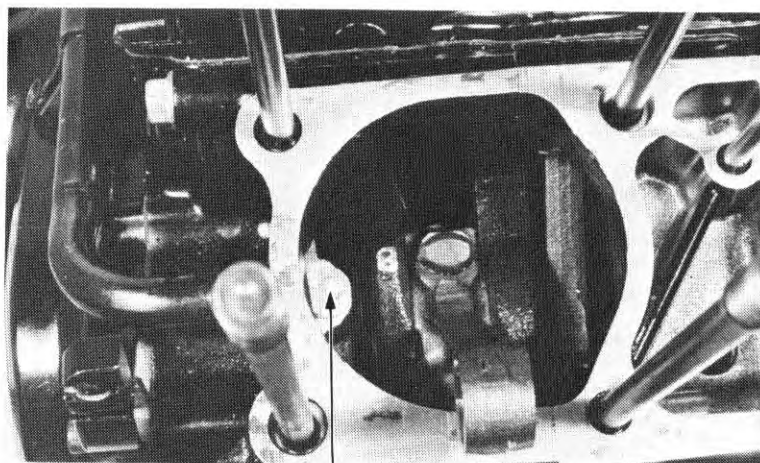
(1) OIL JETS
