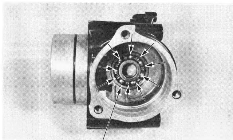
(1) FINAL DRIVEN SHAFT BEARING
