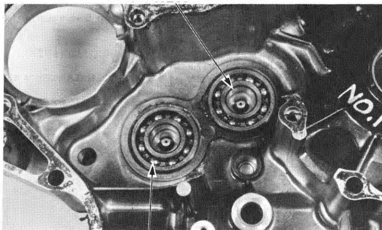
(2) COUNTERSHAFT BEARING
