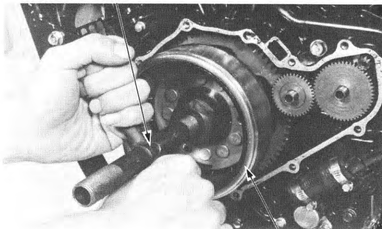
(2) FLYWHEEL
