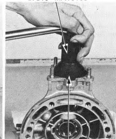
(3) O-RING GUIDE 07973-4630200
