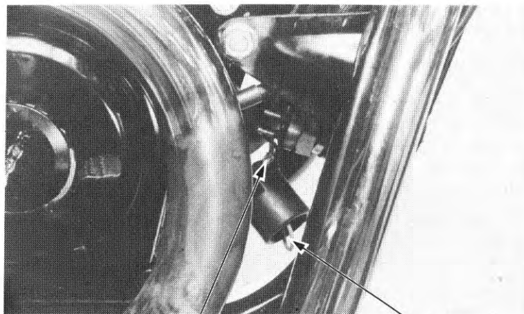
(1) THERMOSTATIC SWITCH LEADS (2) JUMPER WIRE
