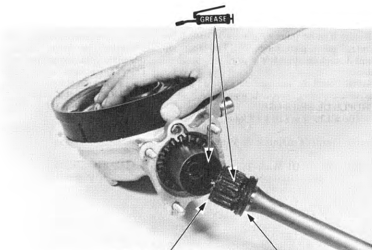
(1) STOP RING
