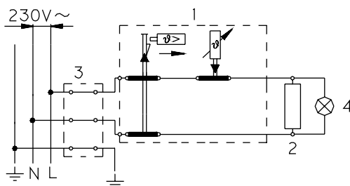
Electric installation
