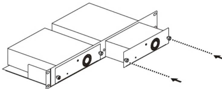
Figure 1.27 –Installing the DPS-200A/500A in the DPS-800
