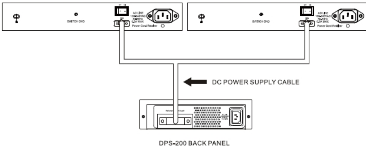
Figure 1.26 – Connecting two Switches to the DPS-200A/500A
