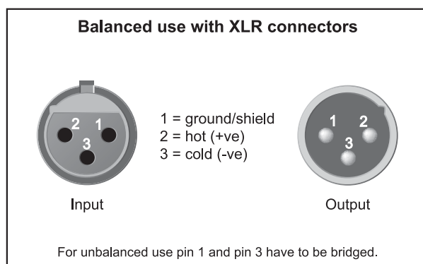
Fig. 8.1: XLR connectors
