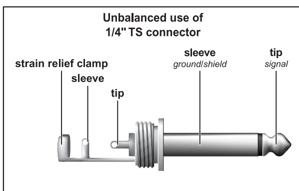
Fig. 8.2: 1/4" mono plug
