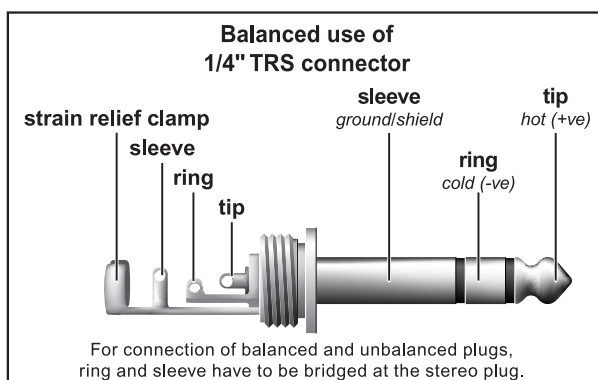
Fig. 8.3: 1/4" stereo plug
