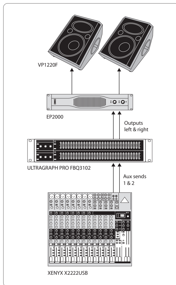
Fig. 3.2: The ULTRAGRAPH PRO FBQ3102 in a monitor system
