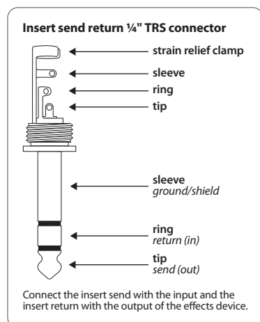
Fig. 4.4: ¼" TRS connector for insert send/return applications
