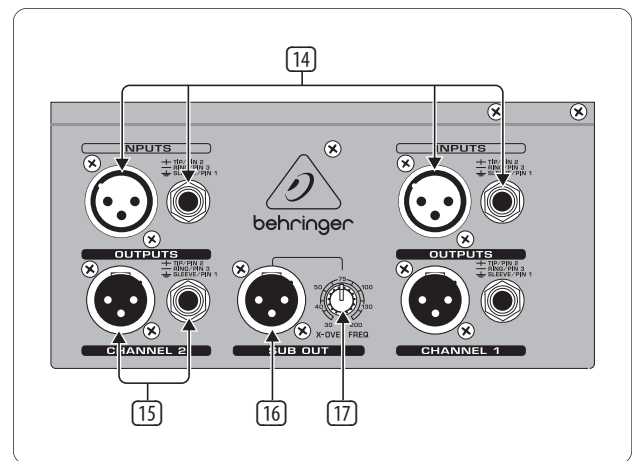
Fig. 2.3: Connectors at the rear of the FBQ3102
