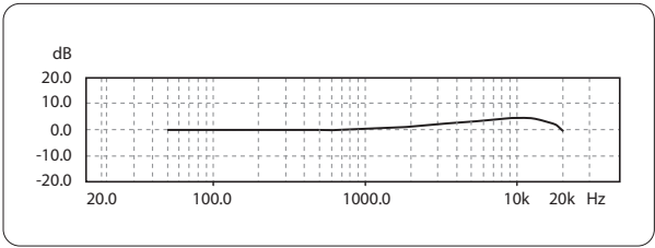
Frequency response
