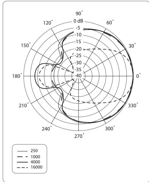
Polar pattern
