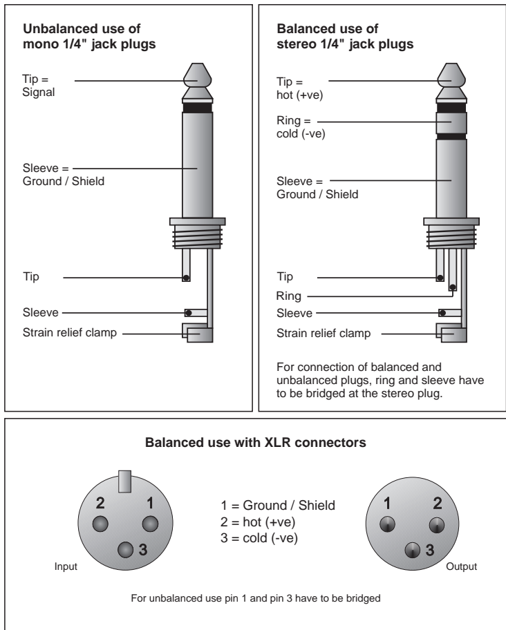
Fig. 3.2: Different plug types
