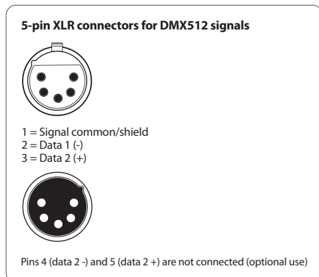
Fig. 4.1: Pin assignment of a 5-pin XLR connector
